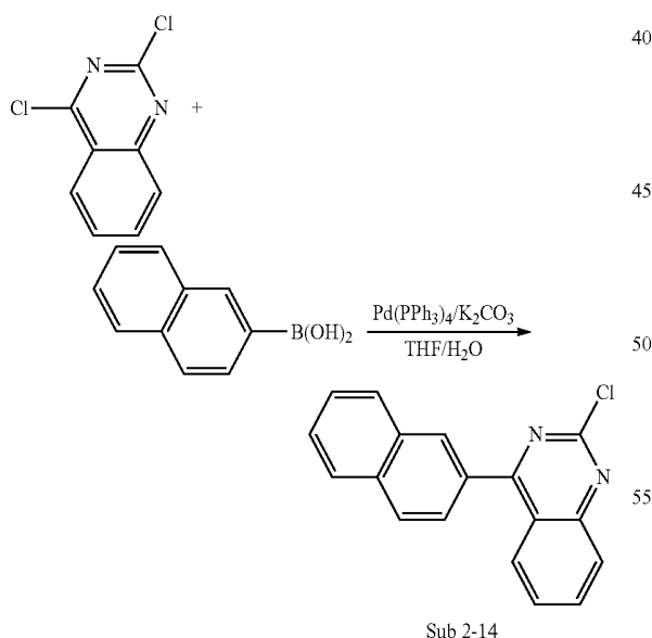
&lt;Reaction Scheme 13&gt;
