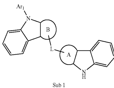
&lt;Reaction Scheme 1&gt;
