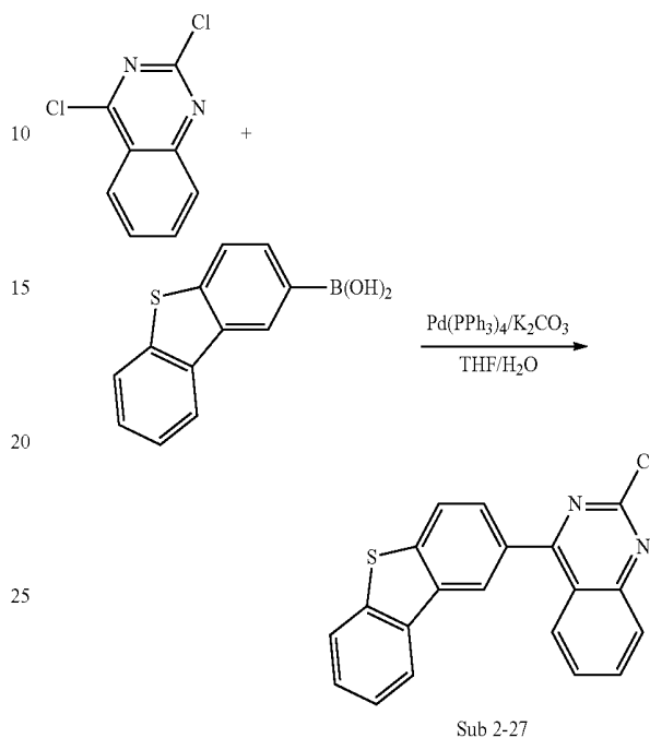
&lt;Reaction Scheme 14&gt;
