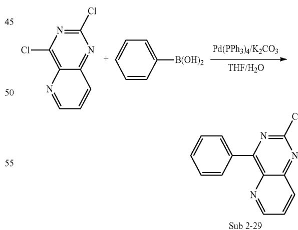
&lt;Reaction Scheme 15&gt;
